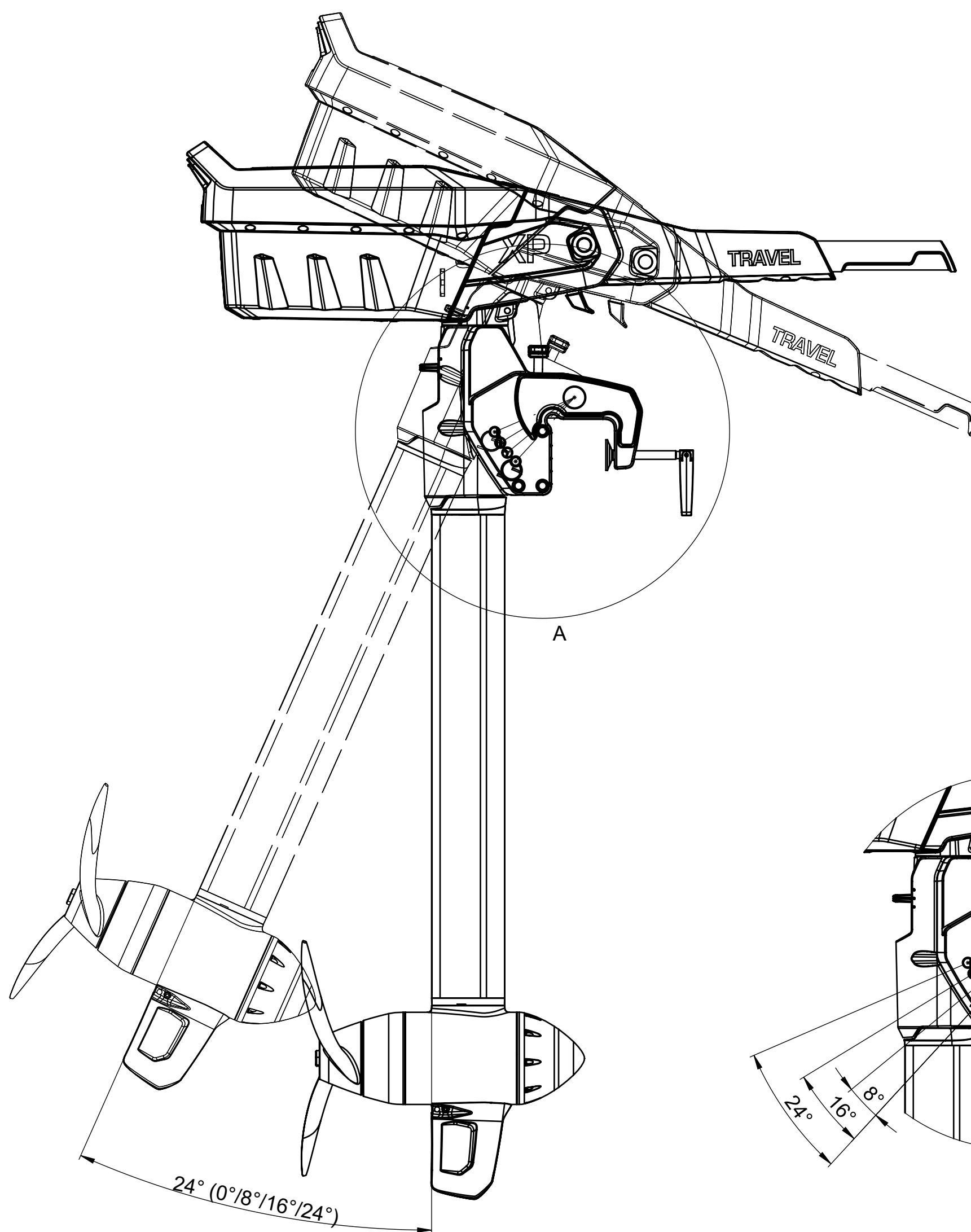
Trim Position / Trim Position
