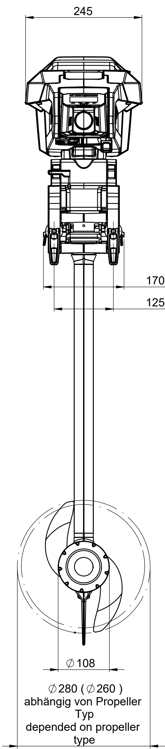
Front View / Frontansicht
