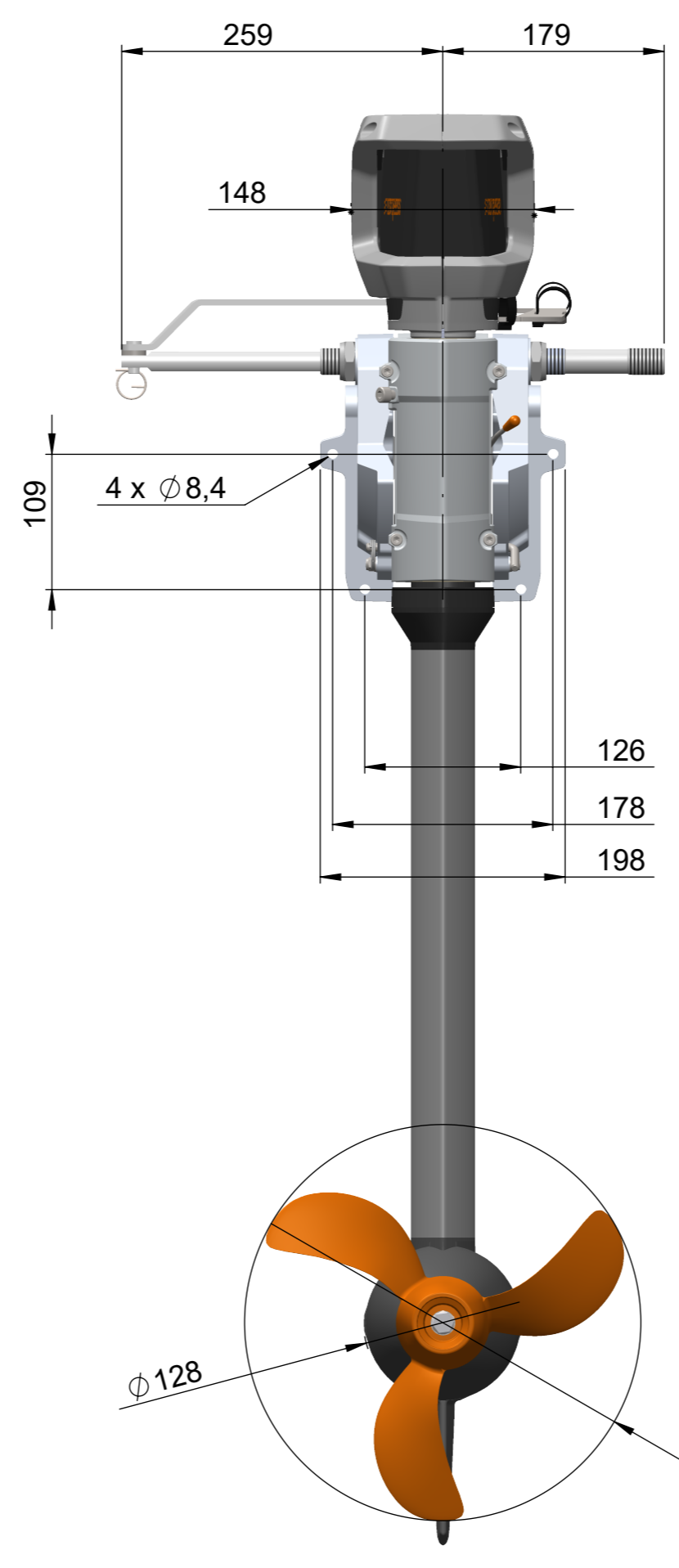
Cruise 6.0 Standard Propeller B 12,5x17 HSP [1987-00]
