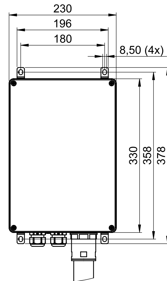
DETAIL A
